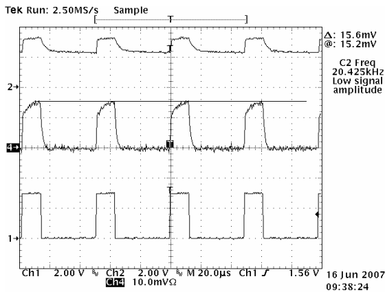
PWM Minimum duty cycle 15 \mu S 20kHz CH1: PWM Signal CH2: Anode of LED CH4: LED current 10mA/div
