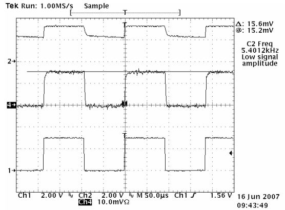
PWM 50% Duty Cycle 5kHz
