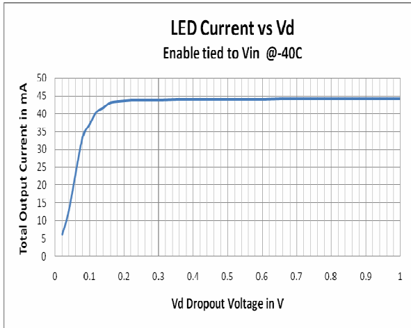
I OUT is for 3 Channels 15mA per channel
